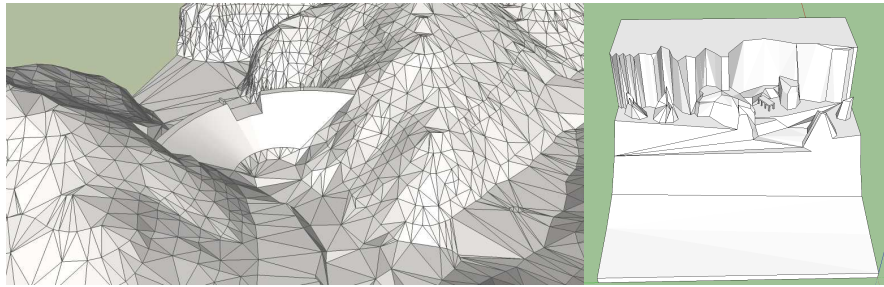
Fig. 1. Design of the computational domain using Google SketchUp software: environment of a dam (left), a rocky bay (right) .
