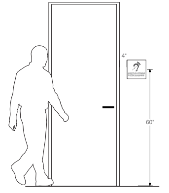
Mounting Guidelines Type O (Wall - Hallway Side) Sign to mount with VHB foam tape and silicone
