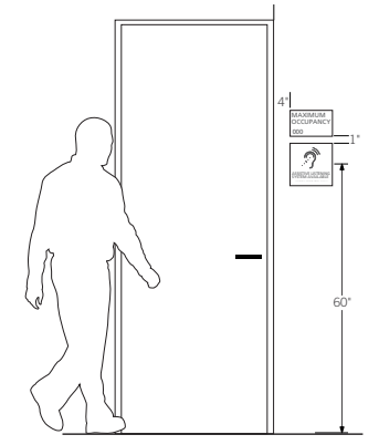
Mounting Guidelines Type P (Interior wall - Occupant Side) Sign to mount with VHB foam tape and silicone
