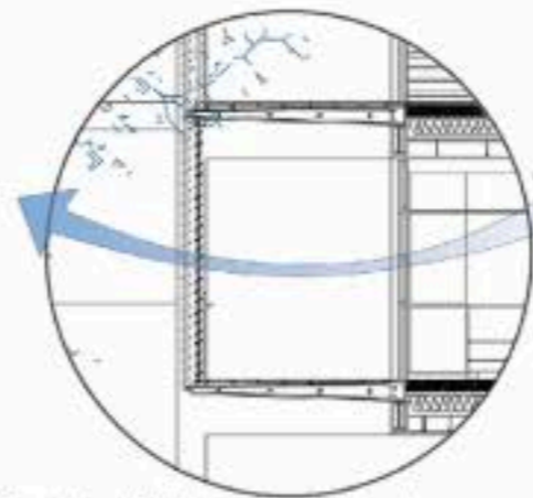
Sectional Filters including louver system, glass, and shading devices
